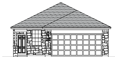
ELEVATION A (with stone)
